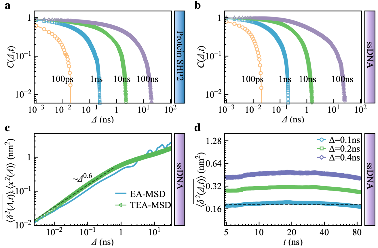
Fig. 4 Control simulation on a single-stranded DNA (ssDNA). The normalized autocorrelation functions (Supplementary Equation 6) of distance fluctuation were obtained from molecular dynamics simulations for different trajectory lengths (i.e., 100 ps, 1 ns, 10 ns, 100 ns). Both (a) protein SHP2 and (b) ssDNA show non-converged dynamics. (c) MD-derived EA-MSD (blue) vs. TEA-MSD (green) for the ssDNA. (d) TEA-MSD of ssDNA as a function of observation time, t , with three fixed lag times \Delta .
